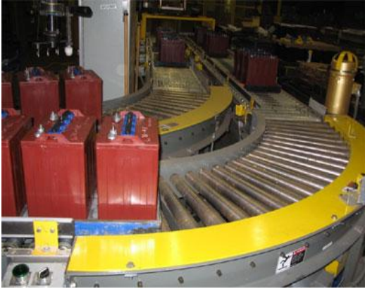
Zone roller conveyor system for batteries
